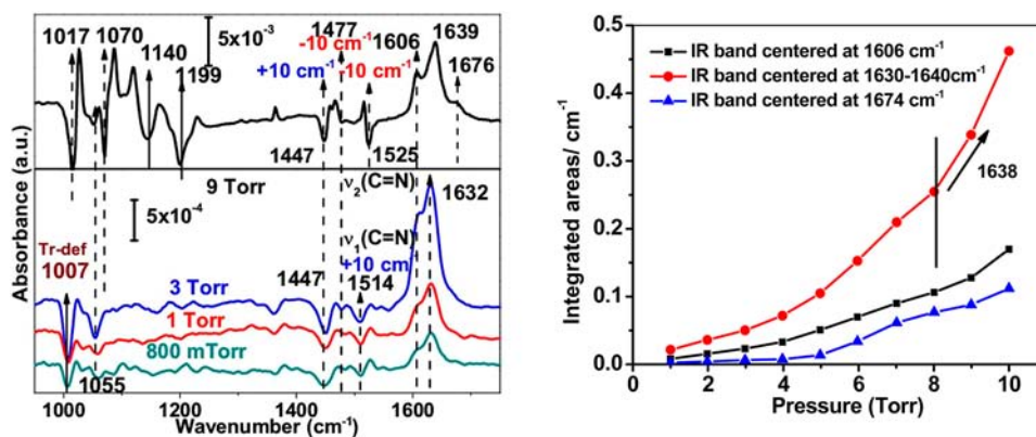
Figure 3. Left: IR absorption spectra of \text{H}_2\text{O} adsorbed in FMOF-1 showing the bending modes of adsorbed water as a function of pressure. Top part shows IR absorption spectrum at 9 Torr. Right: Integrated area of the bending modes as a function of pressure.
